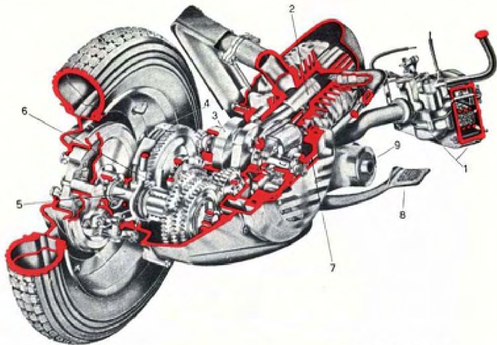
Fig. 5 - Engine section
